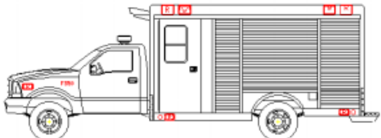
SD0778FP – 2-door forward personnel – 108"CA – 67.5' turning radius
