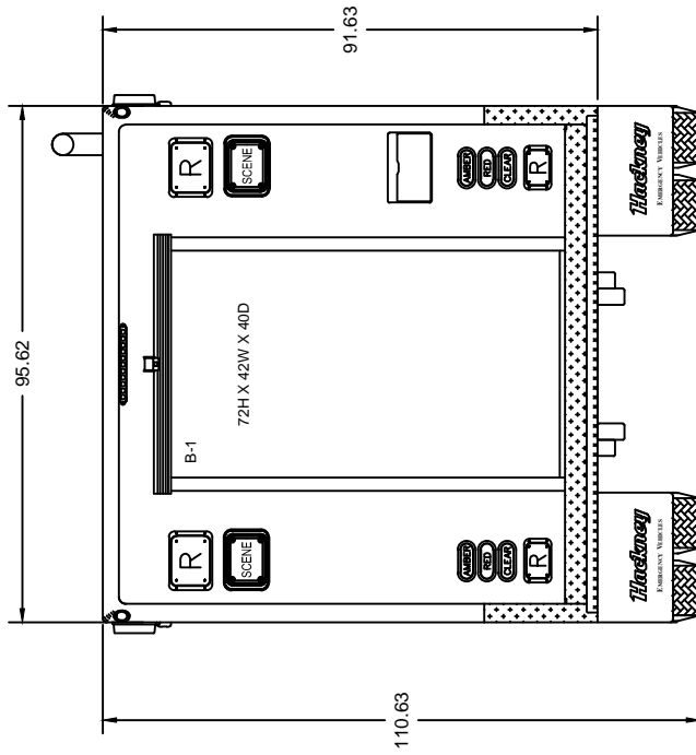
REAR VIEW
